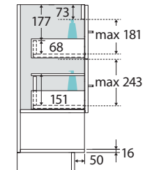
SIDE VIEW: DRAWER STORAGE
