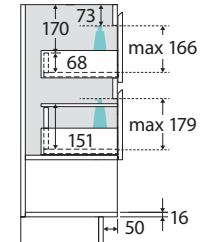
SIDE VIEW: DRAWER STORAGE
