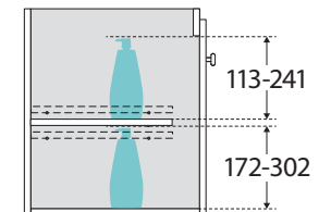
SIDE VIEW: SHELF STORAGE (Adjustable)
