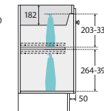
SIDE VIEW: SHELF STORAGE (Adjustable)
