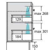
SIDE VIEW: DRAWER STORAGE
