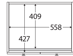
SIDE VIEW: SHELF STORAGE (Adjustable)
