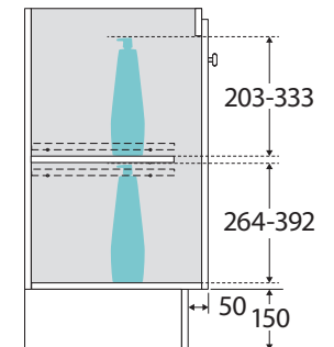
SIDE VIEW: SHELF STORAGE (Adjustable)
