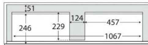
TOP VIEW: DRAWER AREA (Dimensions may vary depending on basin position)
