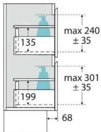
SIDE VIEW: DRAWER STORAGE
