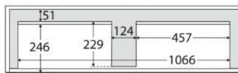
TOP VIEW: DRAWER AREA (Dimensions may vary depending on basin position)
