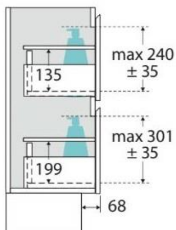
SIDE VIEW: DRAWER STORAGE
