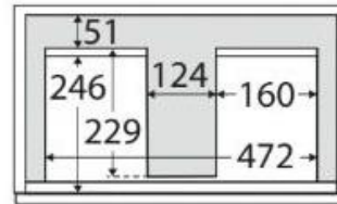
TOP VIEW: DRAWER AREA (Dimensions may vary depending on basin position)
