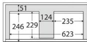
TOP VIEW: DRAWER AREA (Dimensions may vary depending on basin position)
