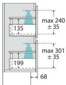
SIDE VIEW: DRAWER STORAGE
