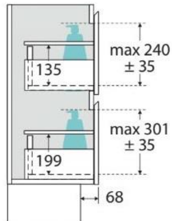
SIDE VIEW: DRAWER STORAGE
