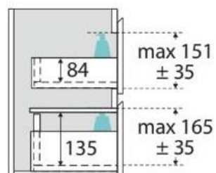
SIDE VIEW: DRAWER STORAGE
