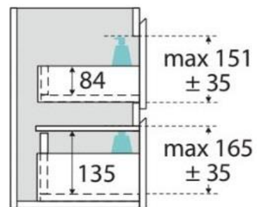
SIDE VIEW: DRAWER STORAGE
