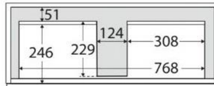
TOP VIEW: DRAWER AREA (Dimensions may vary depending on basin position)
