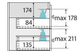
SIDE VIEW: DRAWER STORAGE
