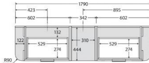
SIDE VIEW: DRAWER STORAGE
