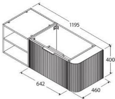
Cabinet with Undermount Basins
