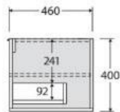
Cabinet with Above Counter or Semi Inset Basins
