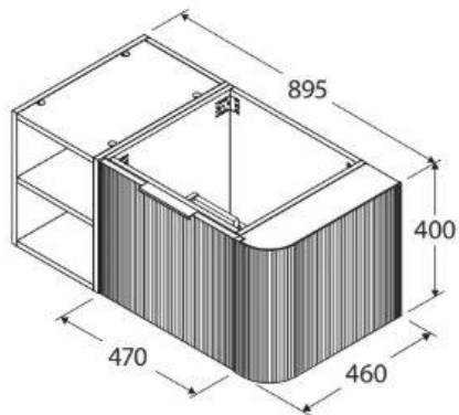
Cabinet with Above Counter or Semi Inset Basins
