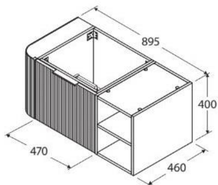
Cabinet with Undermount Basins
