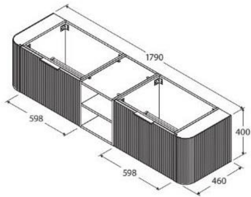
Cabinet with Above Counter or Semi Inset Basins
