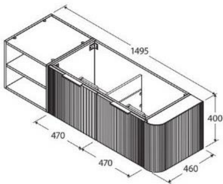
Cabinet with Undermount Basins
