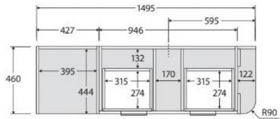
SIDE VIEW: DRAWER STORAGE
