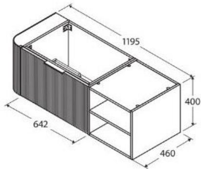
Cabinet with Above Counter or Semi Inset Basins
