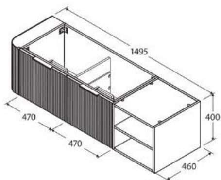
Cabinet with Undermount Basins
