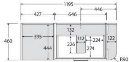
SIDE VIEW: DRAWER STORAGE
