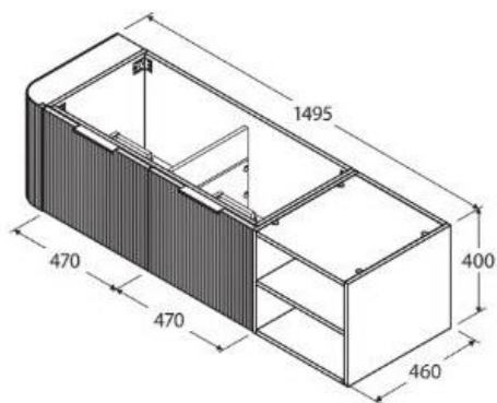
Cabinet with Above Counter or Semi Inset Basins
