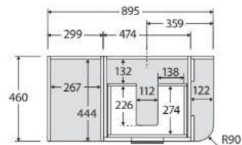
SIDE VIEW: DRAWER STORAGE
