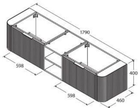
Cabinet with Undermount Basins
