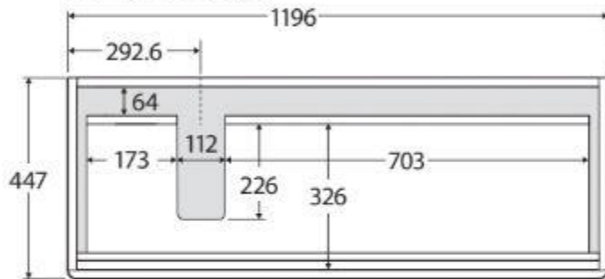
TOP VIEW: CABINET
