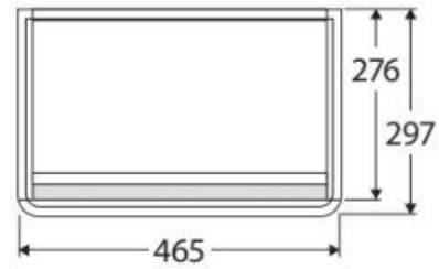
SIDE VIEW: SHELF STORAGE
