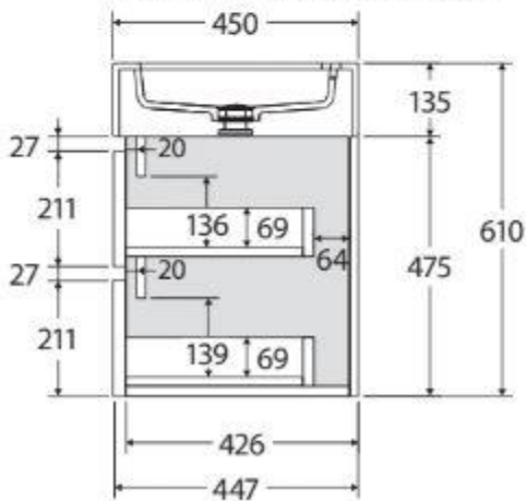
SIDE VIEW: DRAWER STORAGE
