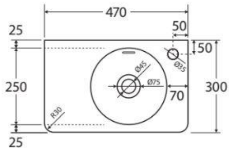
TOP VIEW: BASIN TOP
