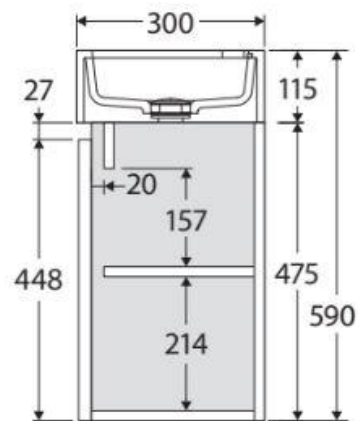
SIDE VIEW: SHELF STORAGE
