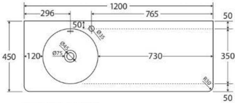
TOP VIEW: CABINET
