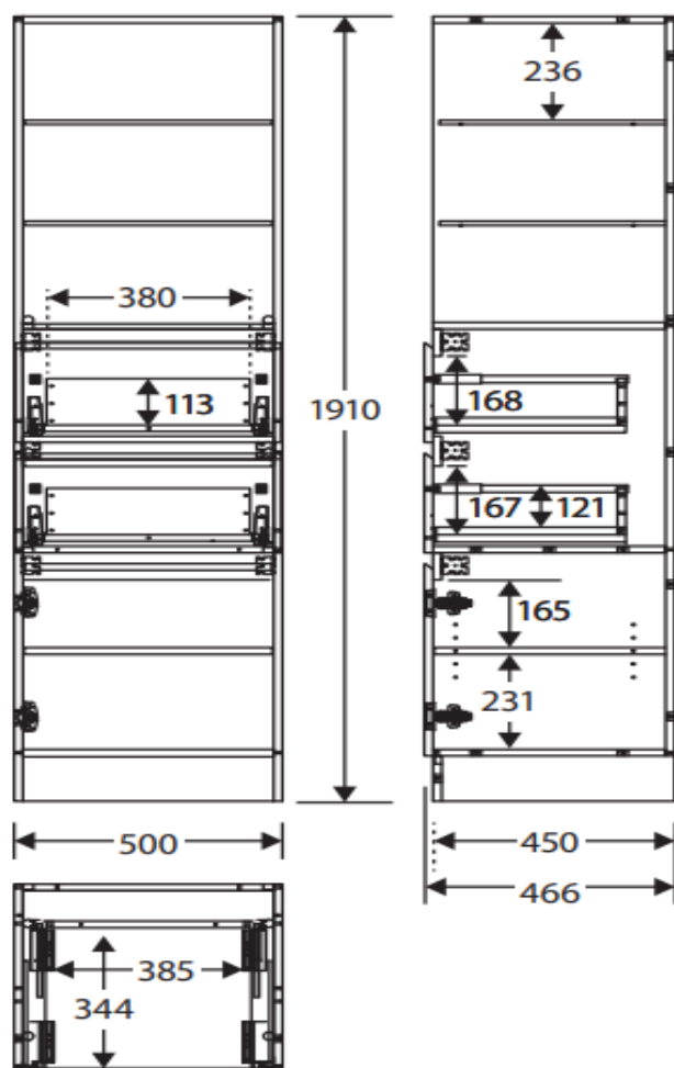
Danelle FLOOR STANDING TALLBOY
