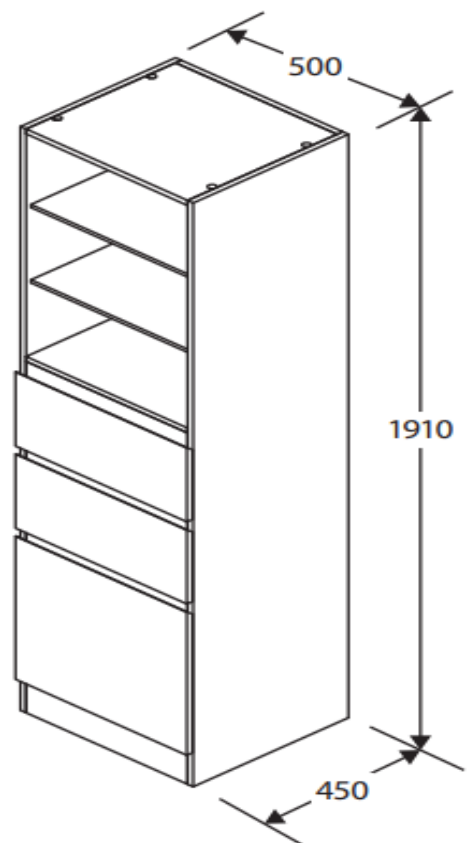
Danelle FLOOR STANDING TALLBOY
